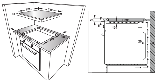
BCF30, BCF30-TZK
