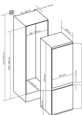
BKG144FKOMBI
