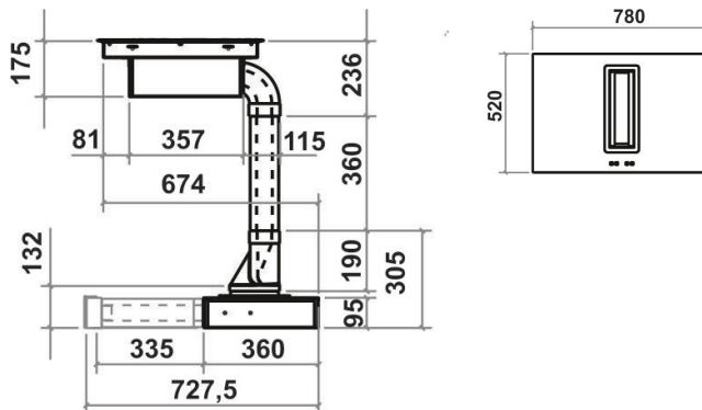
BML78
