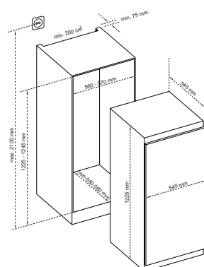
BKS124F, BKG124F
