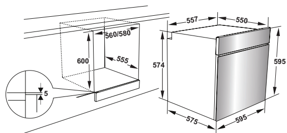
BFK186FD
