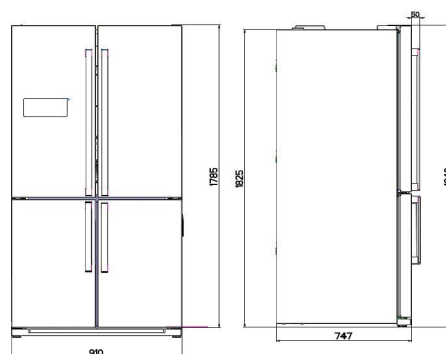
BFK186FD
