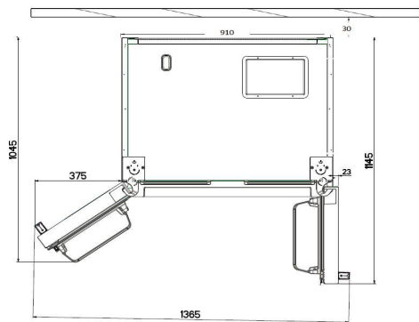
BFK186FD
