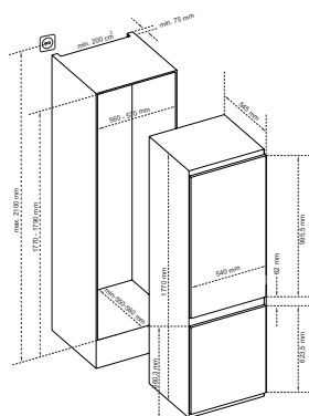
BKG178F, BKG178EMF
