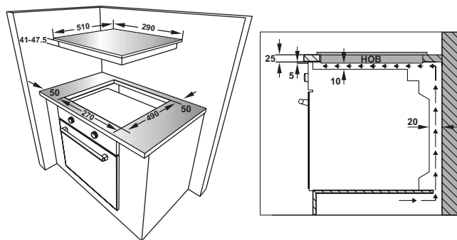
BCF30, BCF30-TZK
